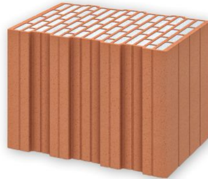
Poroton-S8-P
