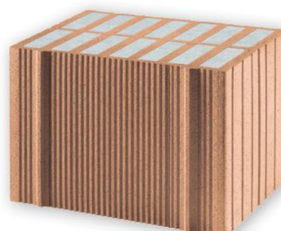
Poroton-S8-P
