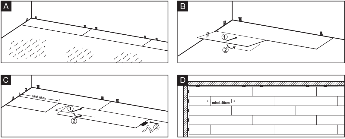
①= insert long tongue, ②= angle in, ③= join ends
